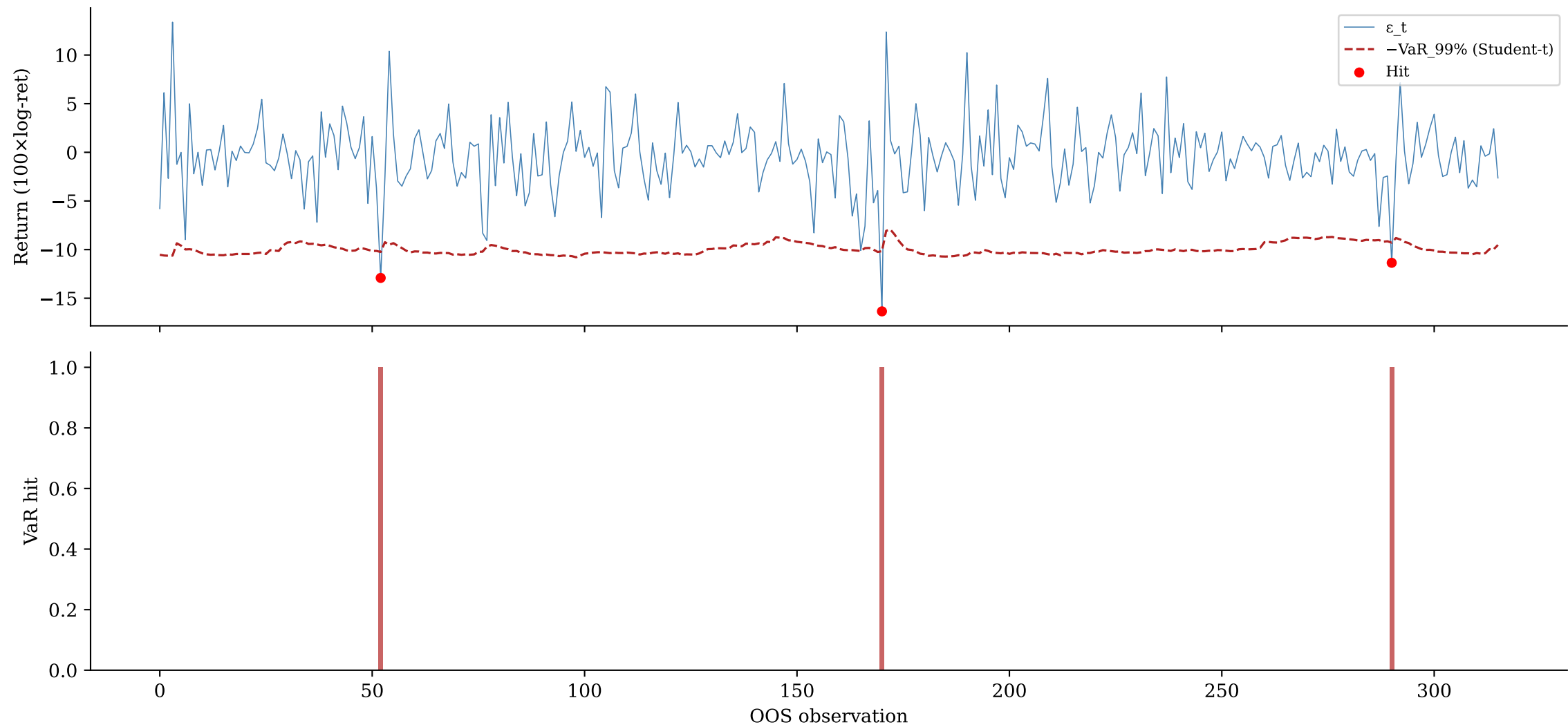
LSTM-SSE-t-Student — ETH-USD VaR 99% Hit Sequence
